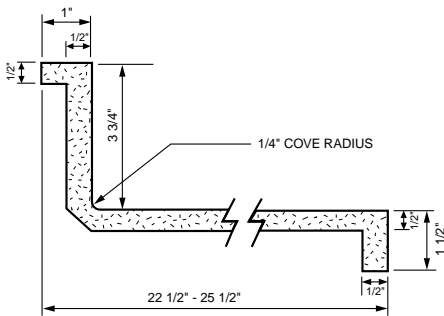
Kitchen and Vanity Top CFV-225, CFK-255
