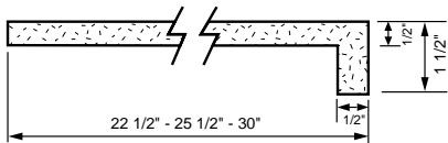
Flat Deck Top CFF-225, CFF-255, CFF-300
